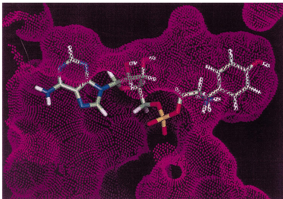
Figure 2. Tyrosinyl adenylate bound in the active site of the Bacillus stearothermophilus tyrosyl tRNA synthetase. A Connolly representation of the enzyme surface is shown by the purple dots. The tyrosine binding pocket and the adenine binding cleft are clearly visible.
