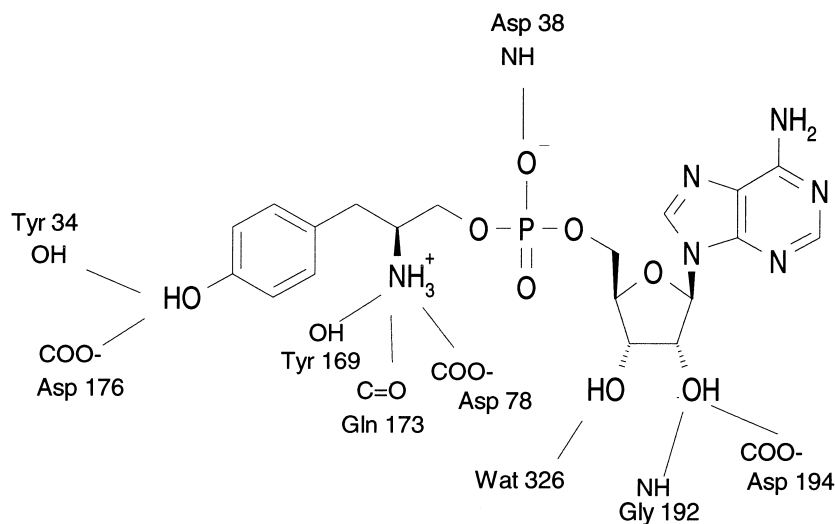
Figure 1. Polar interactions from tyrosinyl adenylate to residues in the active site taken from the X-ray structure. 2
